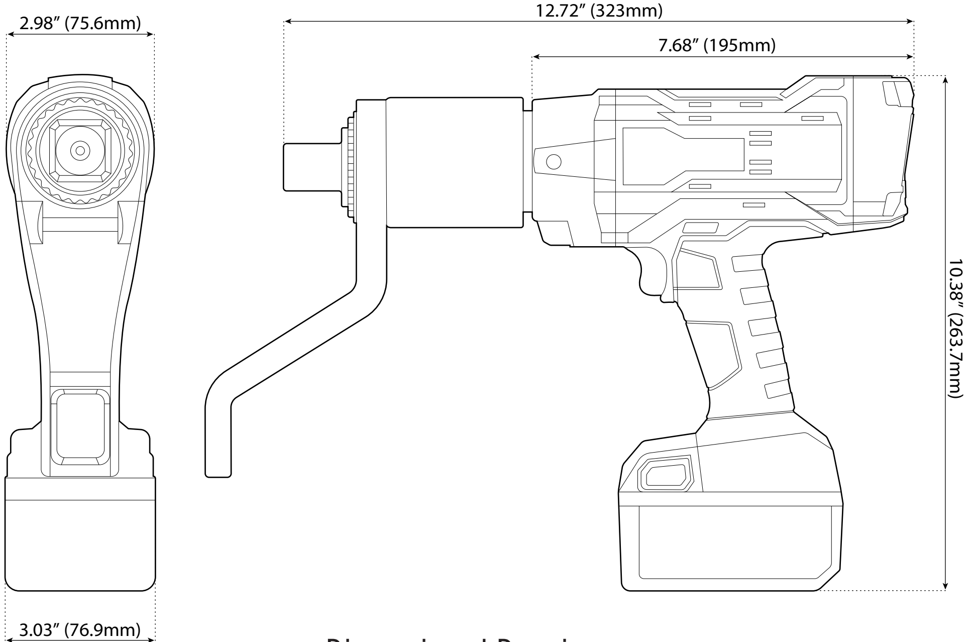
Dimensioned Drawing
