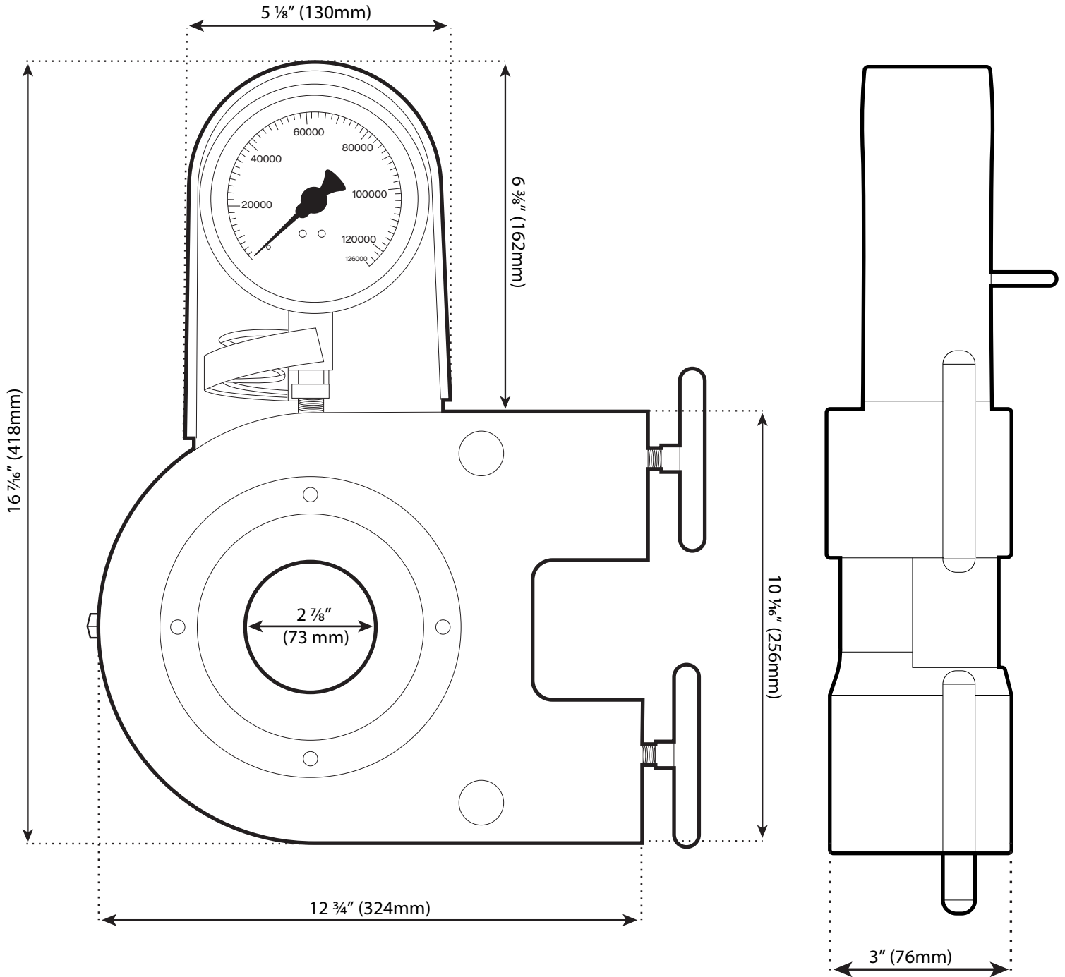
Dimensioned Drawing
