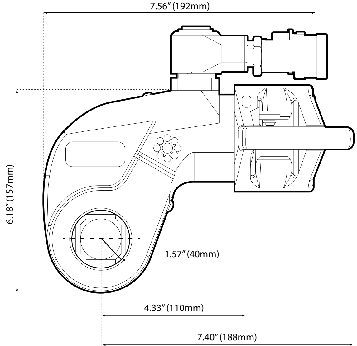
Dimensioned Drawing
