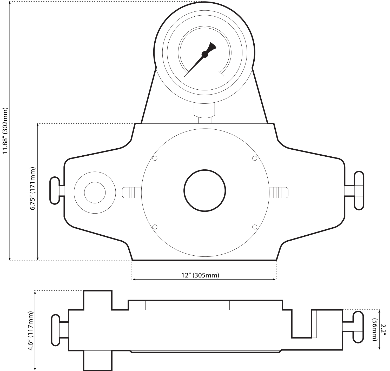
Dimensioned Drawing
