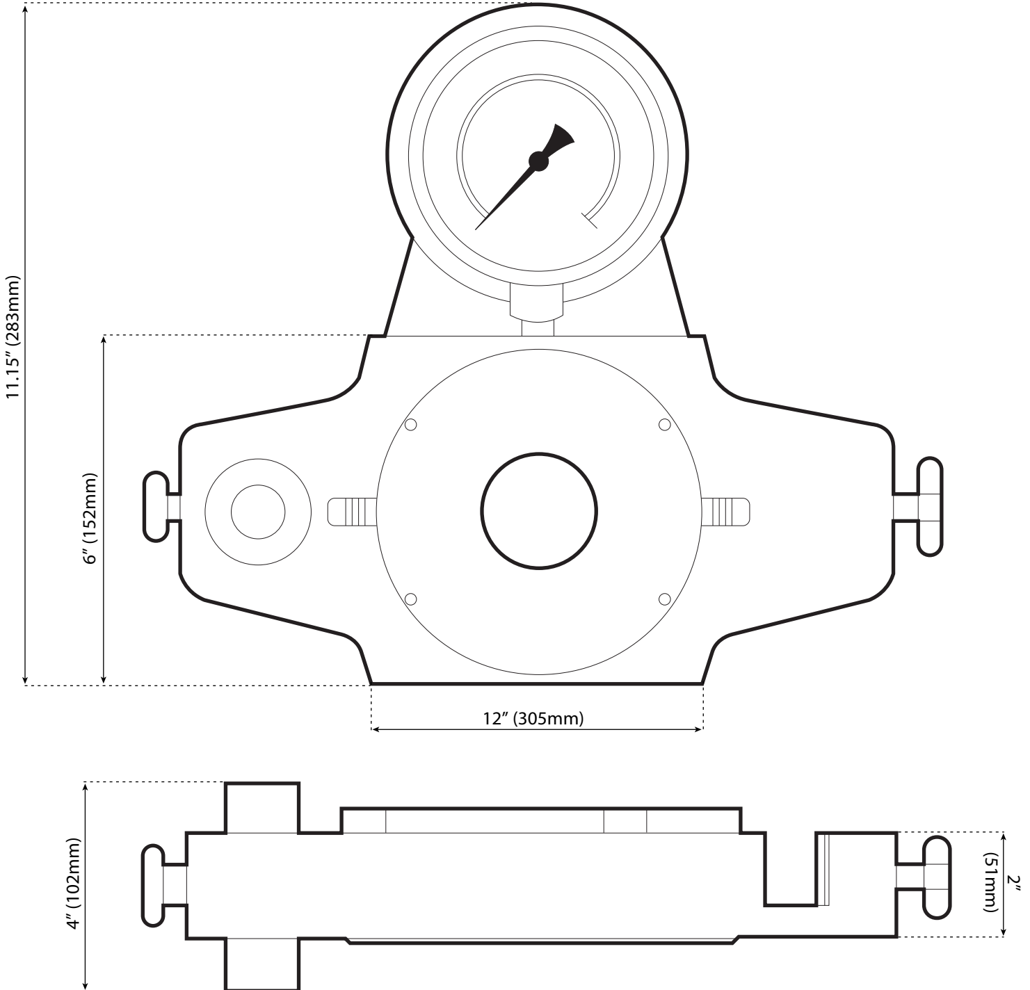
Dimensioned Drawing
