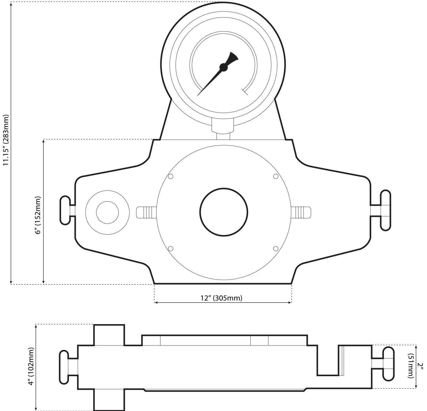
Dimensioned Drawing
