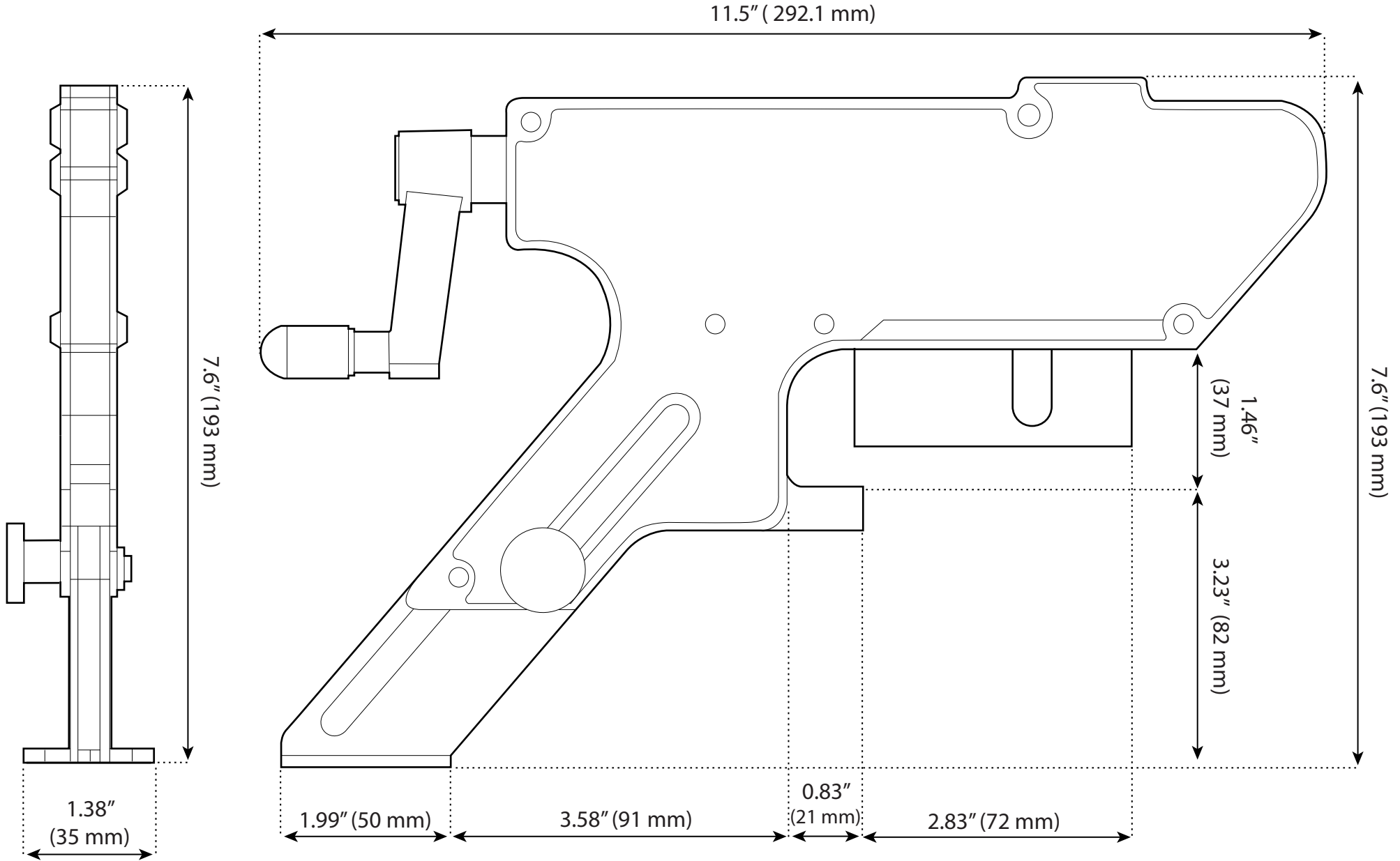
Dimensioned Drawing
