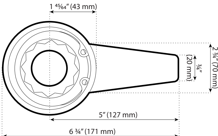
2" Bar Socket– (1 1/4" Bolt Diameter)
