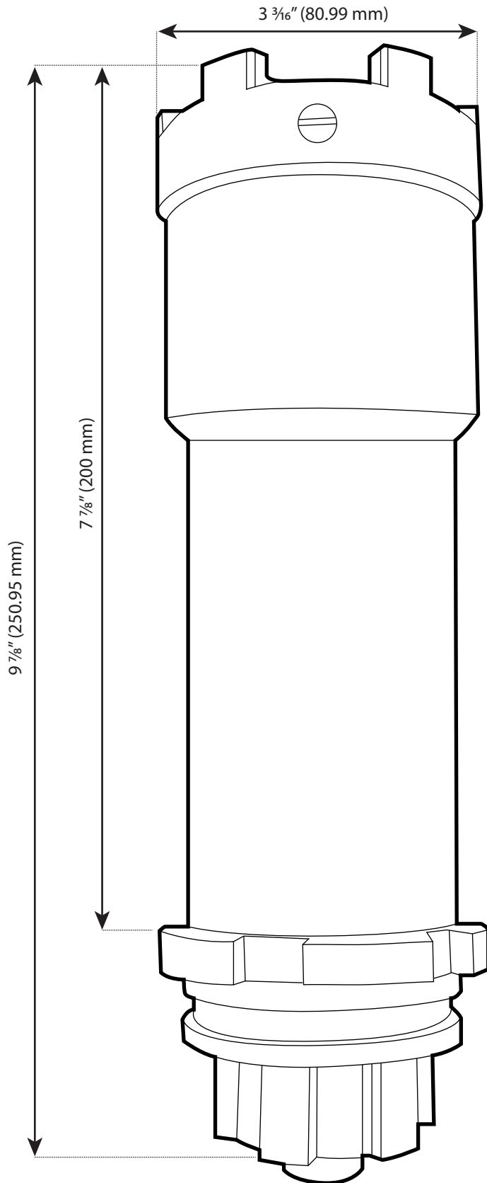
Dimensioned Drawing
