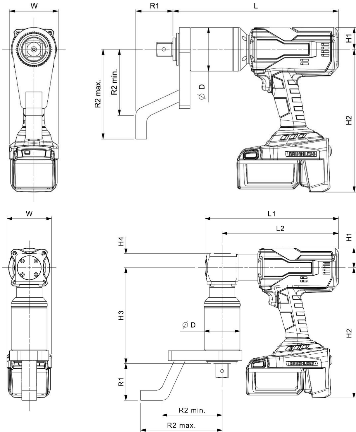
FIGURE 21 – Tool Dimensions
