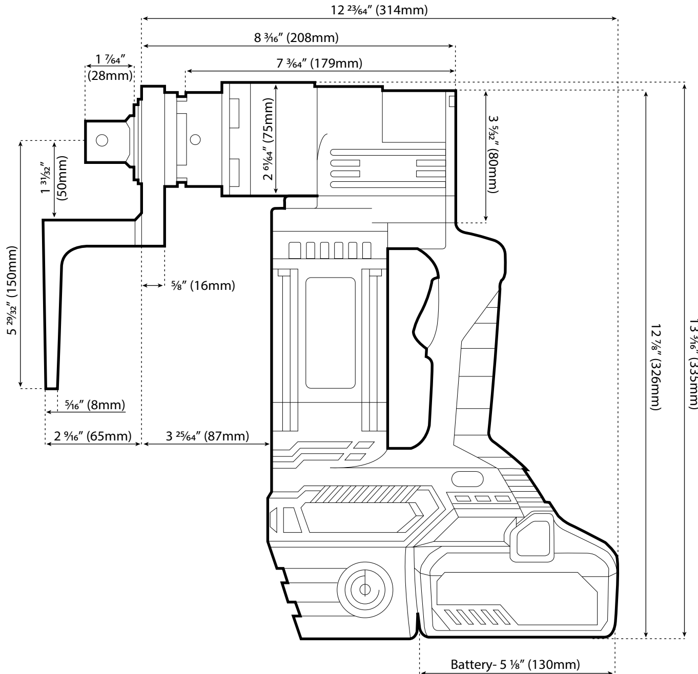
Dimensioned Drawing
