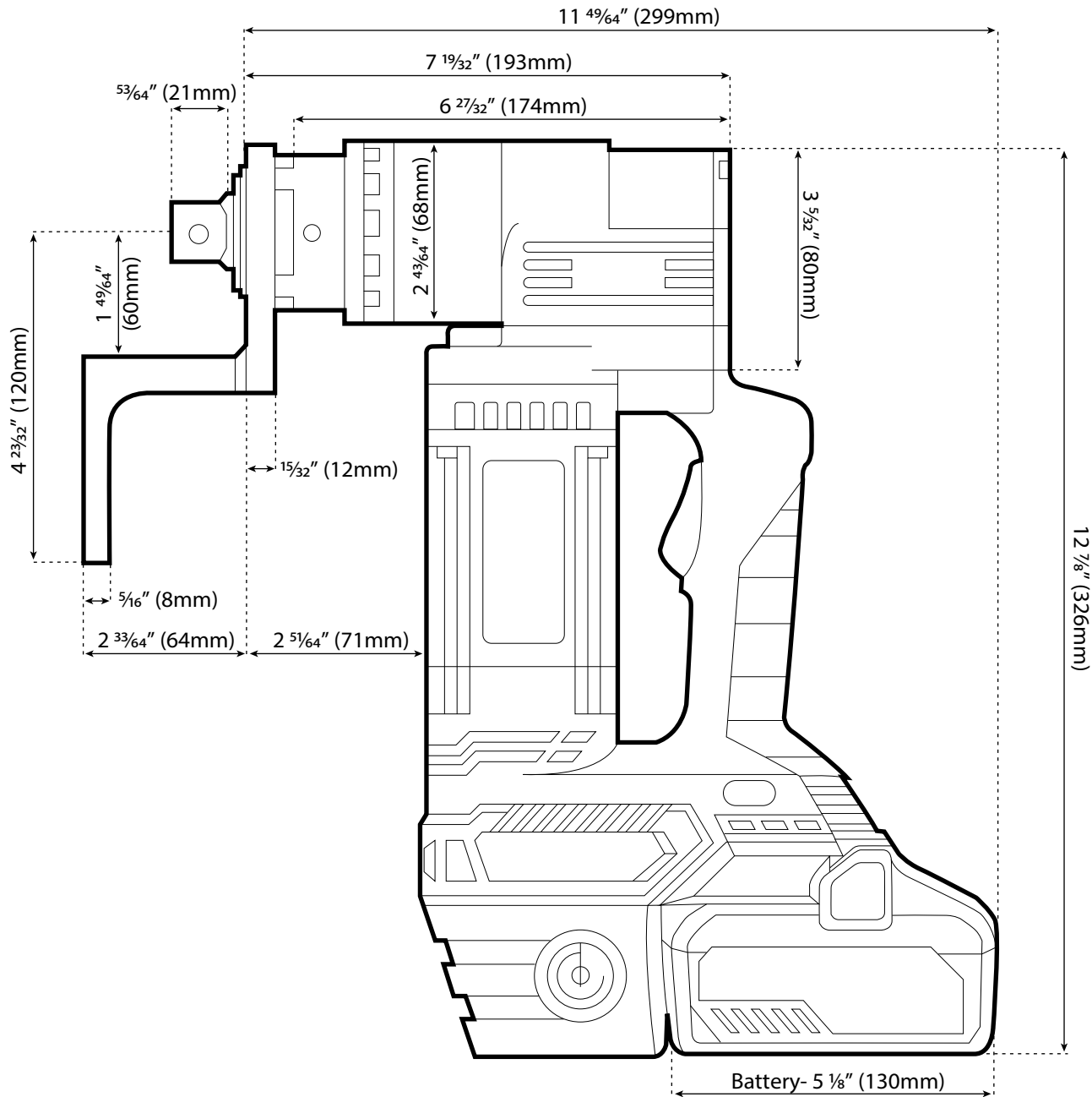
Dimensioned Drawing
