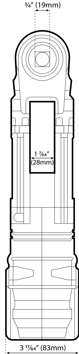
Square Drive w/ Reaction Bar
