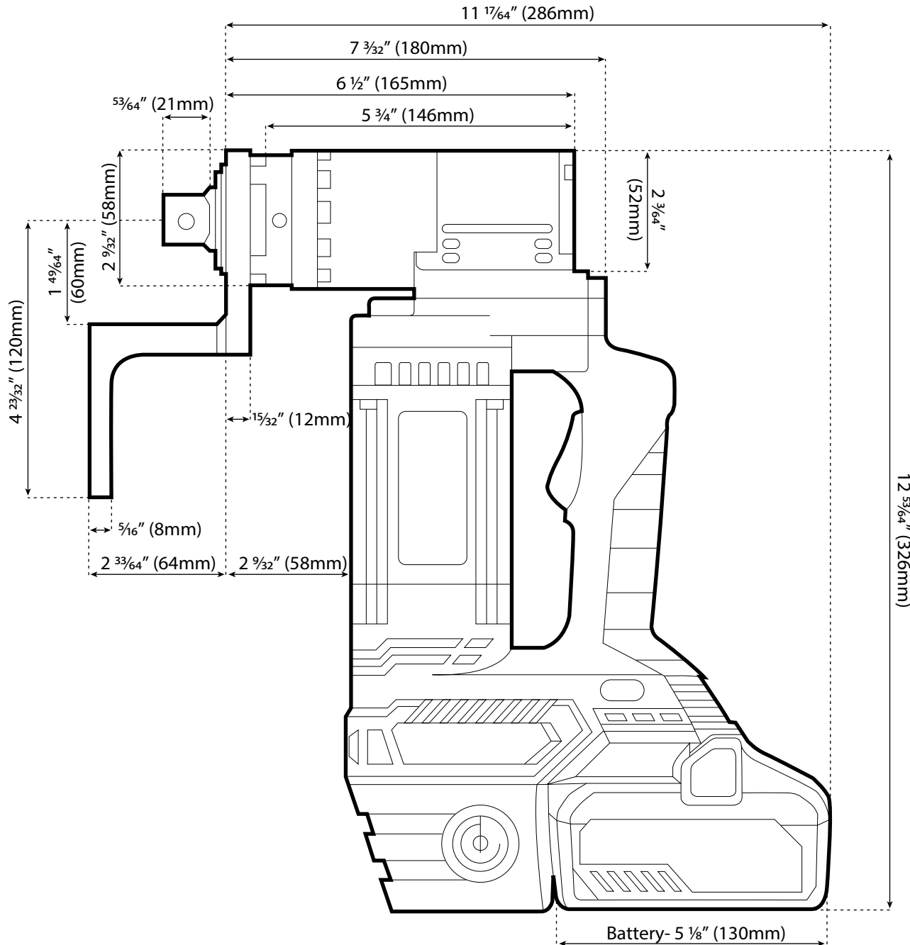
Dimensioned Drawing
