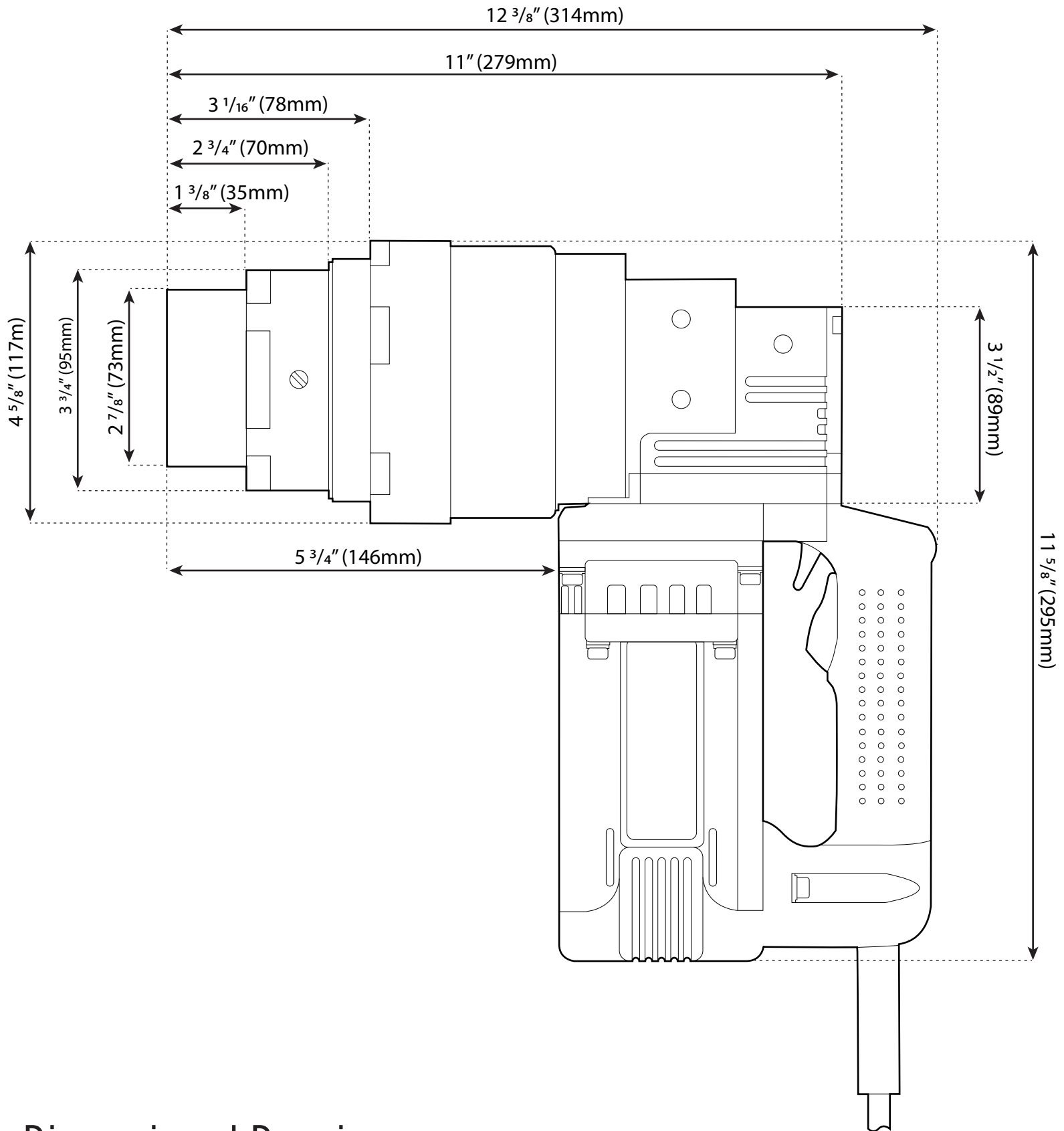
Dimensioned Drawing
