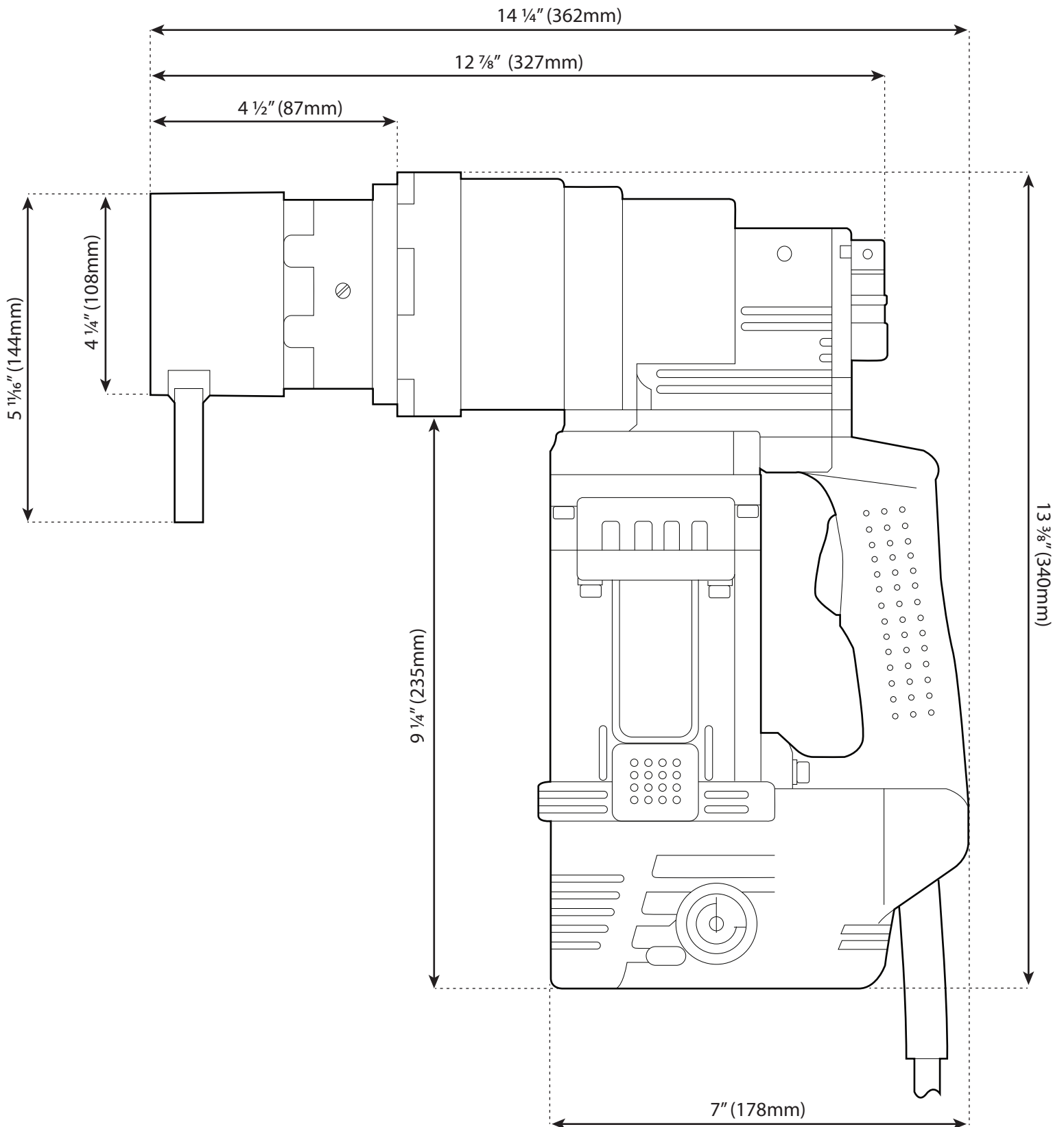
Dimensioned Drawing
