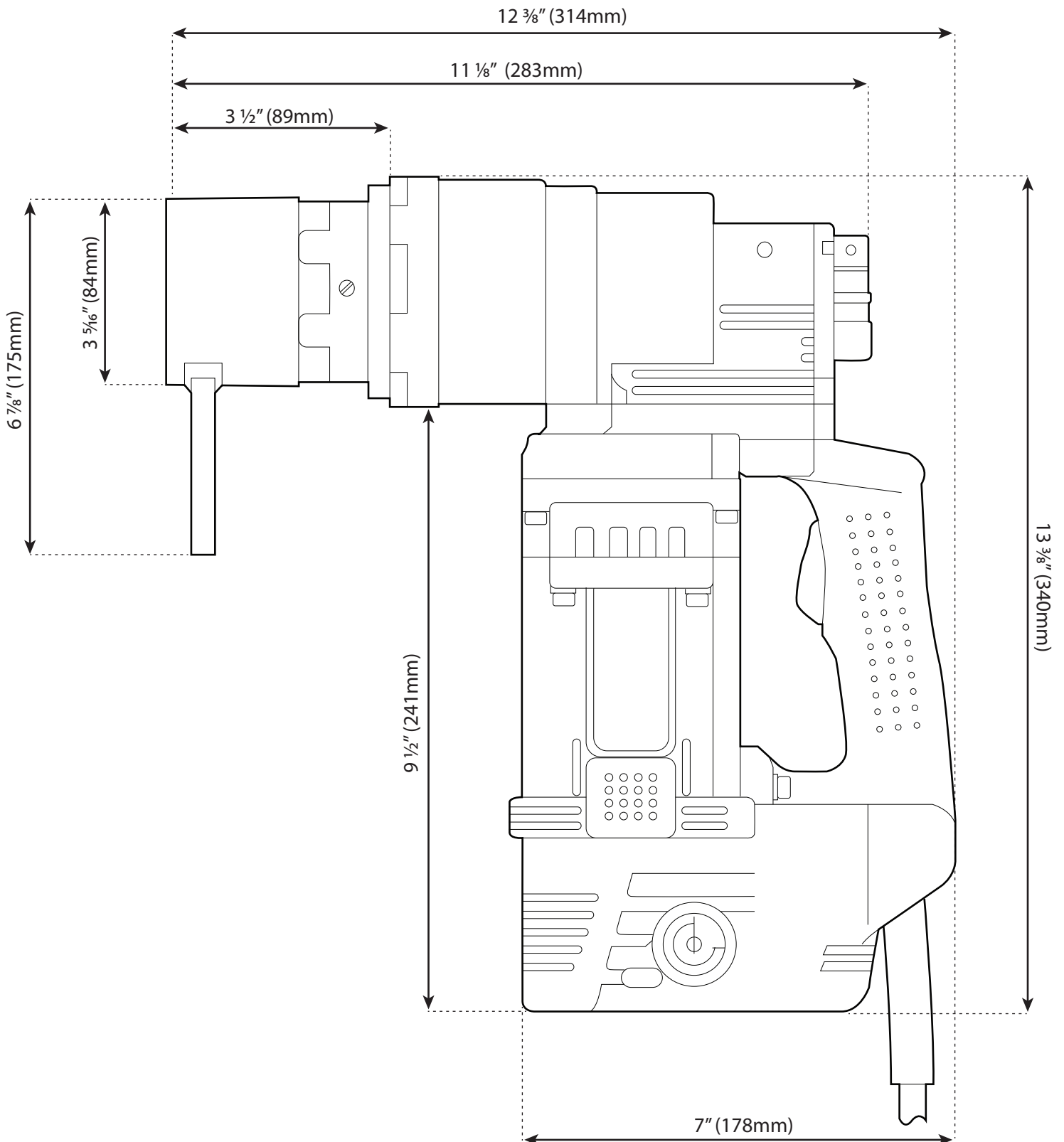
Dimensioned Drawing
