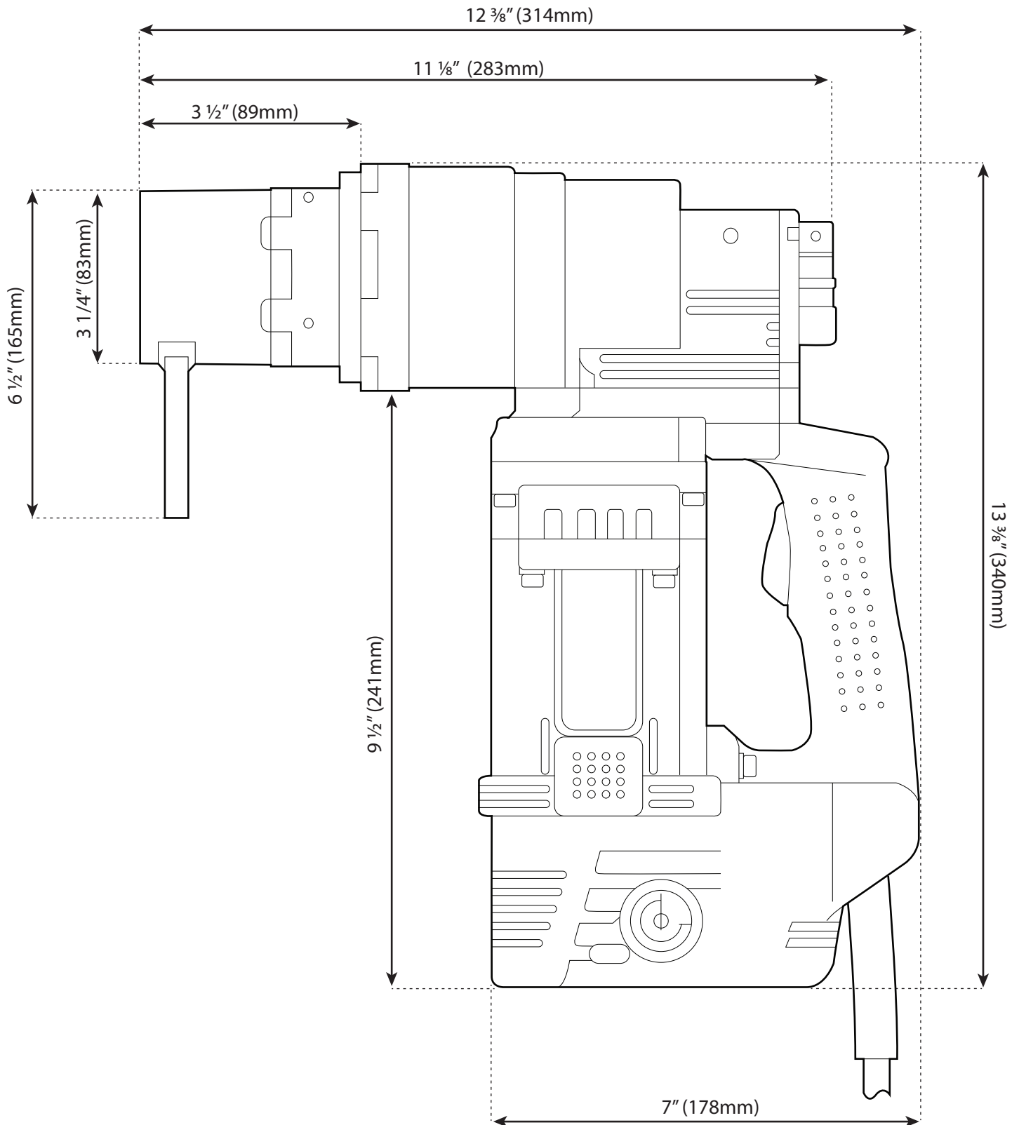
Dimensioned Drawing
