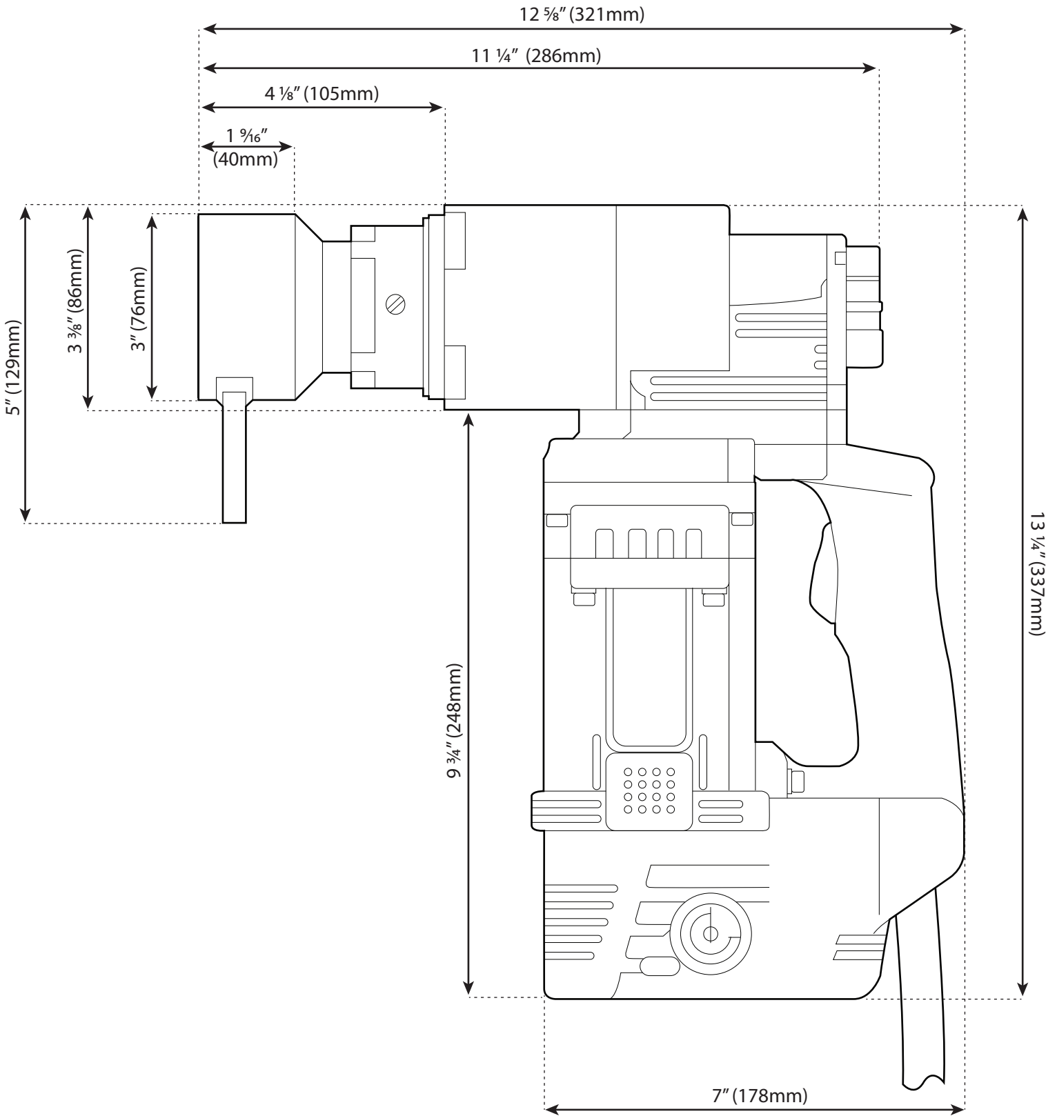
Dimensioned Drawing
