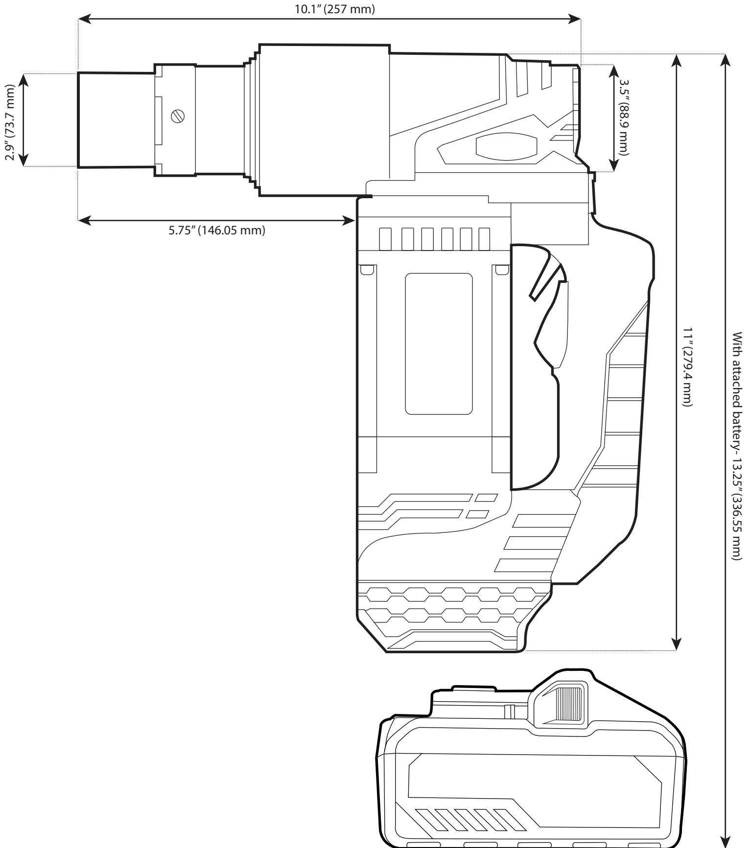
Dimensioned Drawing
