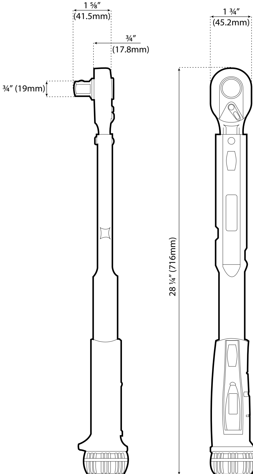
Dimensioned Drawing
