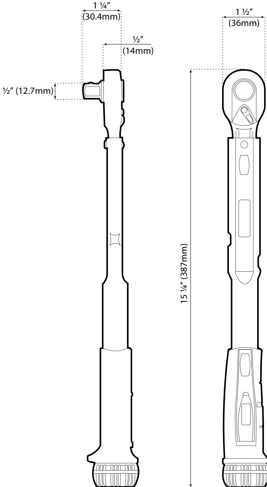
Dimensioned Drawing
