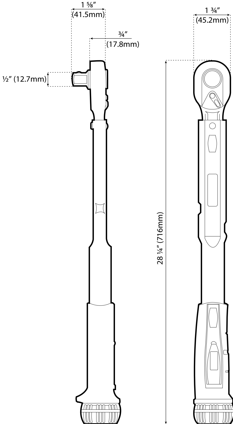
Dimensioned Drawing
