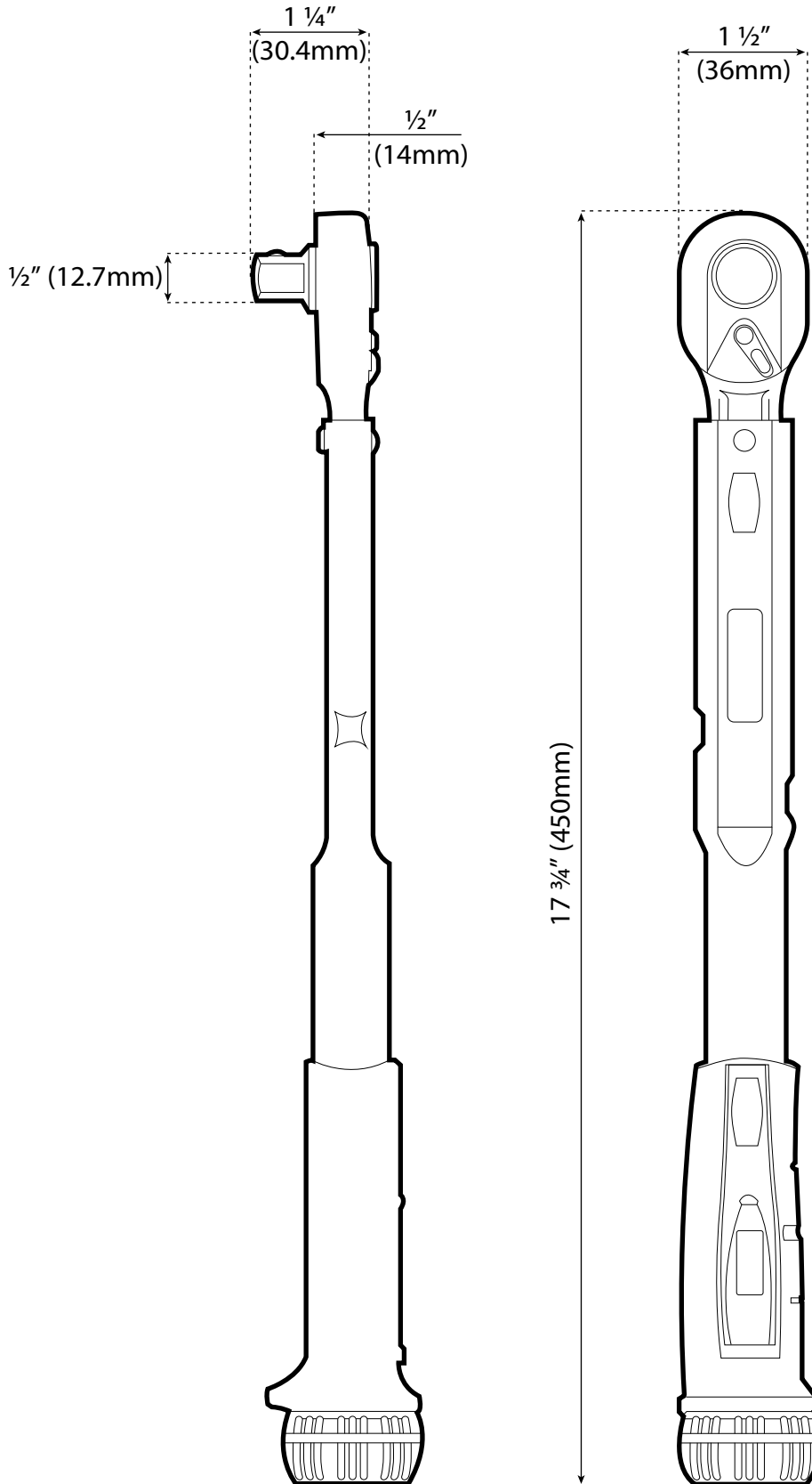
Dimensioned Drawing
