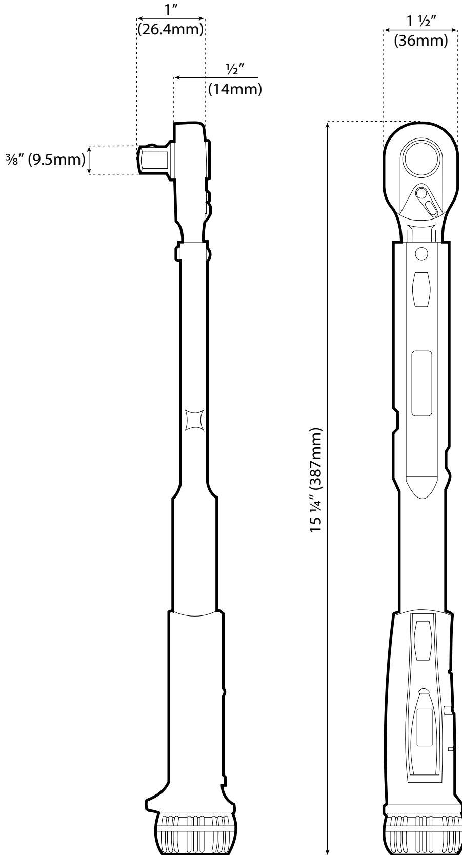
Dimensioned Drawing
