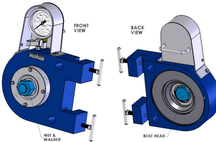
Figure 7, Installation of Fastener Assembly to be Tested
