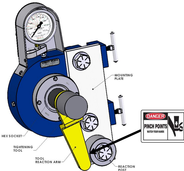
Figure 3, Typical Setup of Torque Reaction Kit
