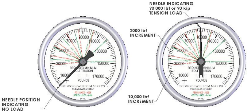
Figure 8, Example of How to Read Gage Dial
