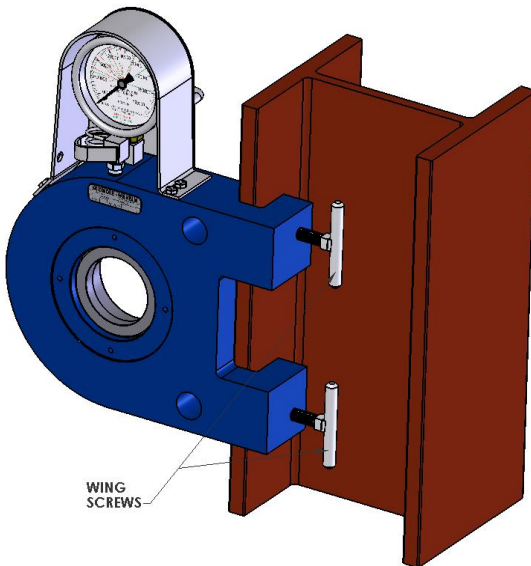
Figure 2, Typical Column Mounting
