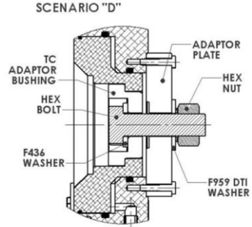
Figure 17, Calibrator Cross-section DTI WASHER PLACED UNDER THE NUT, BOLT IS TURNED TO TIGHTEN
