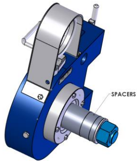
Figure 10, Typical Use of Spacers
