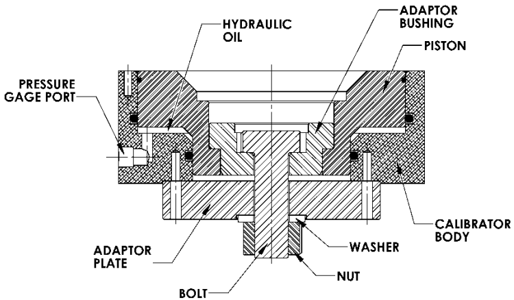
Figure 1, Typical Calibrator Cross-Section
