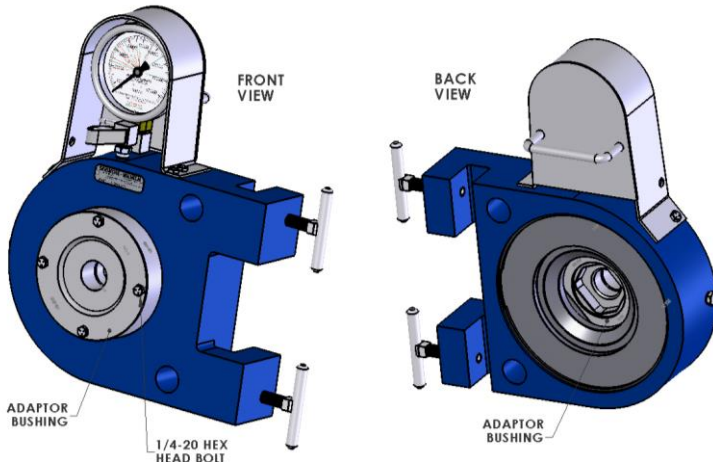
Figure 6, Installation of Adaptor Plate and Bushing
