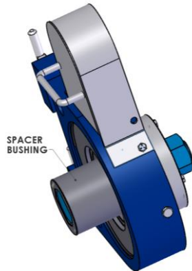
Figure 11, Typical Use of Spacer Bushings
