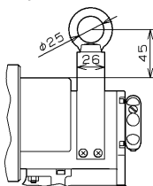
Lifting Device (Optional)
