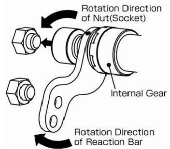
③ Slide impact socket over nut
