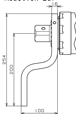
L-type Reaction Bar
