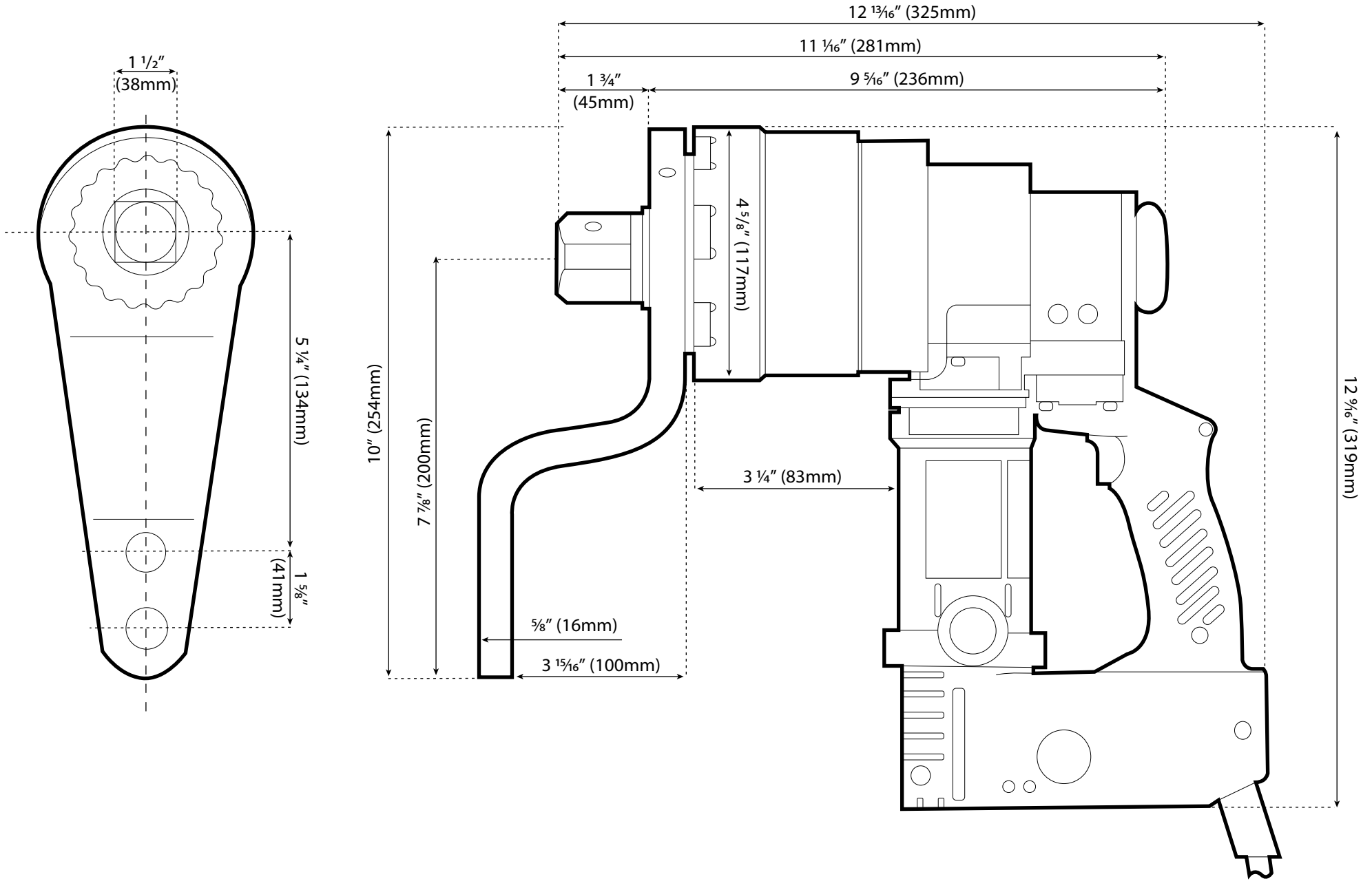
Dimensioned Drawing
