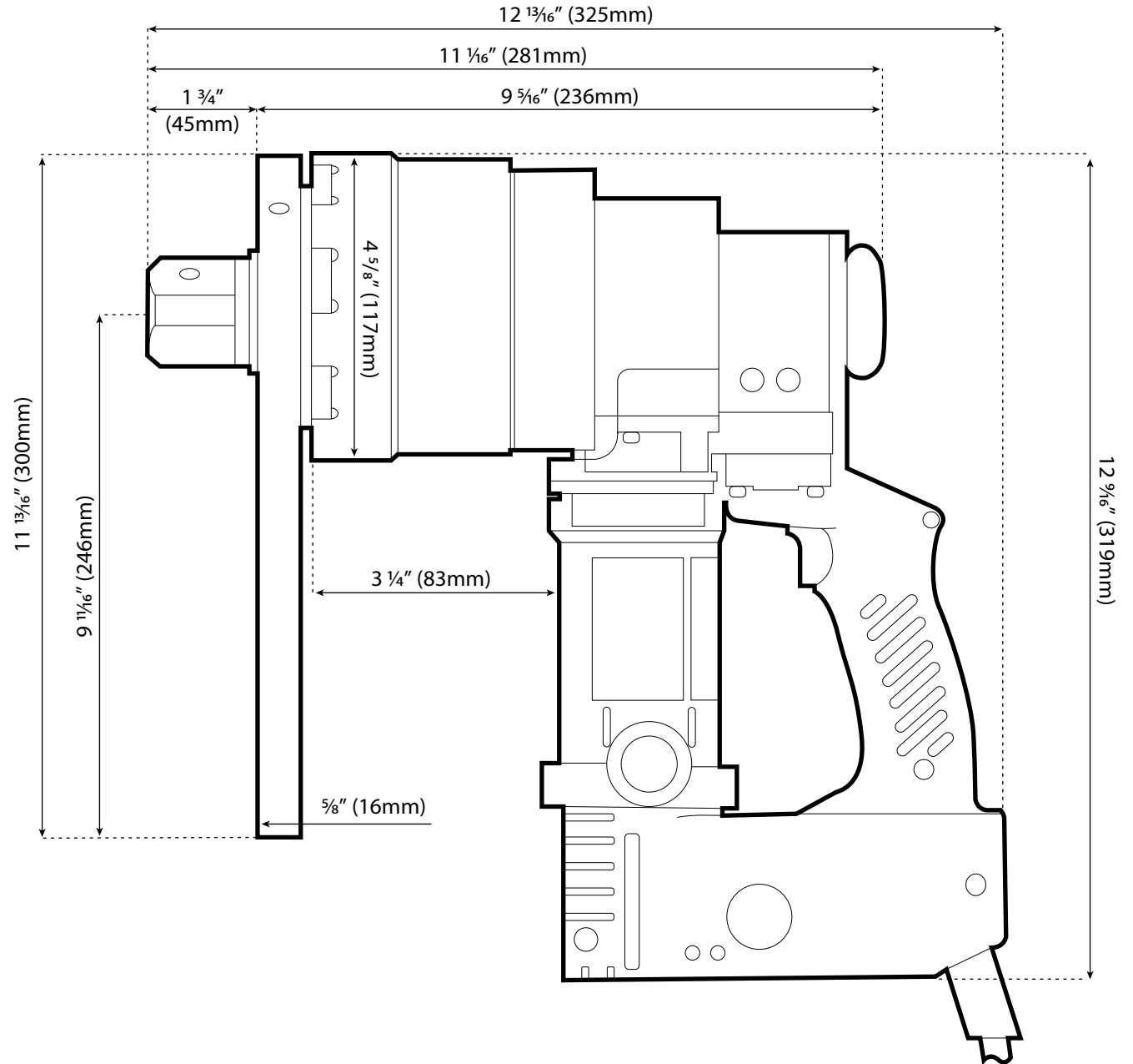
Straight Type Reaction Bar
