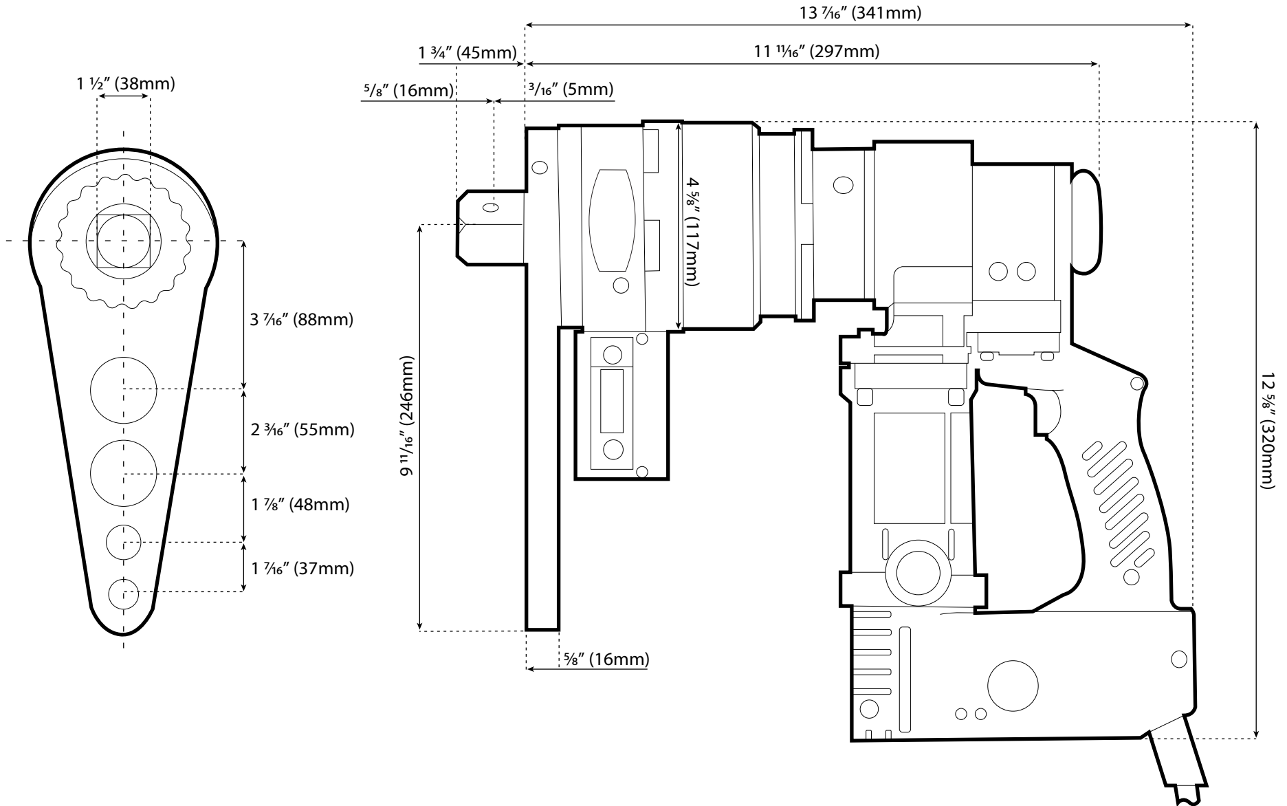
Dimensioned Drawing
