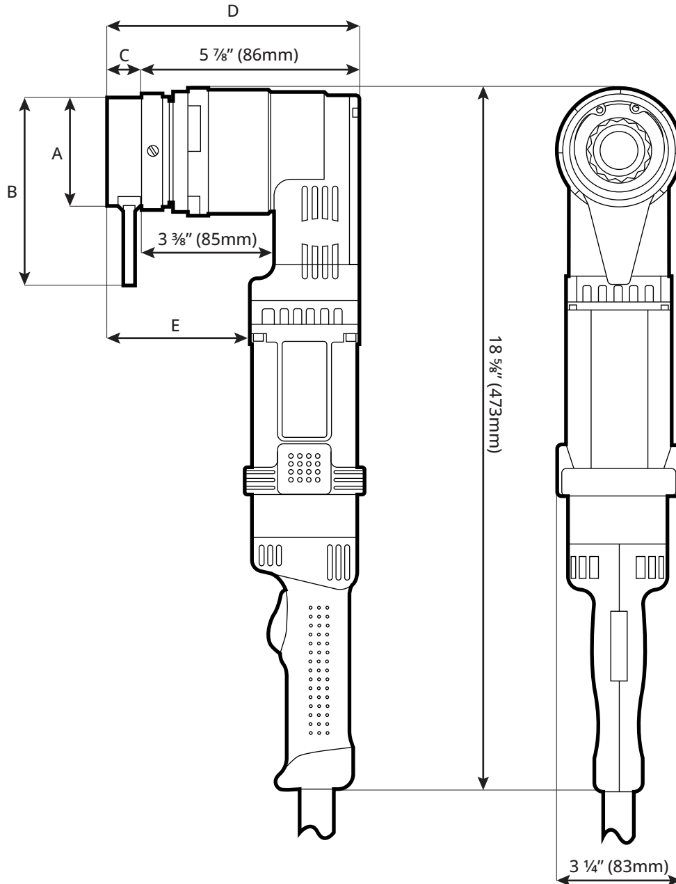
TNC-24EZA Turn-of-Nut Wrench Dimensions w/ Bar Socket
