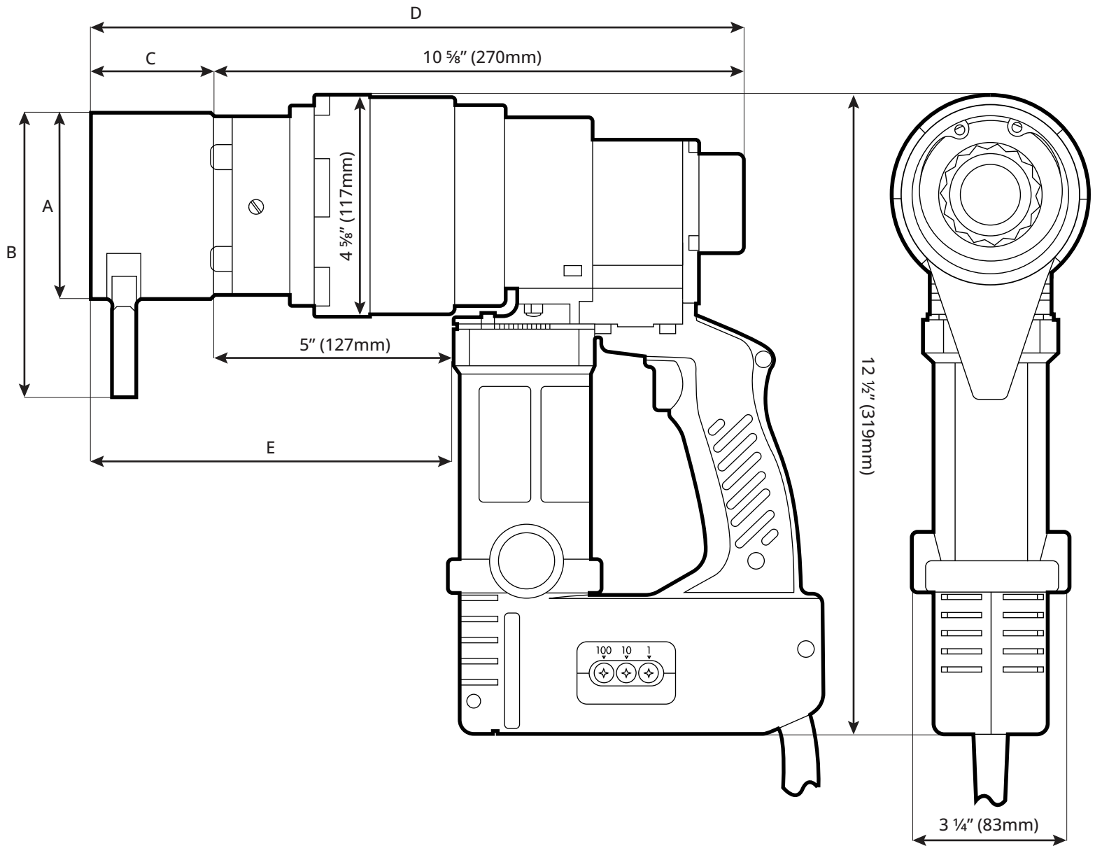
TN-39EZ Turn-of-Nut Wrench Dimensions w/ Bar Socket
