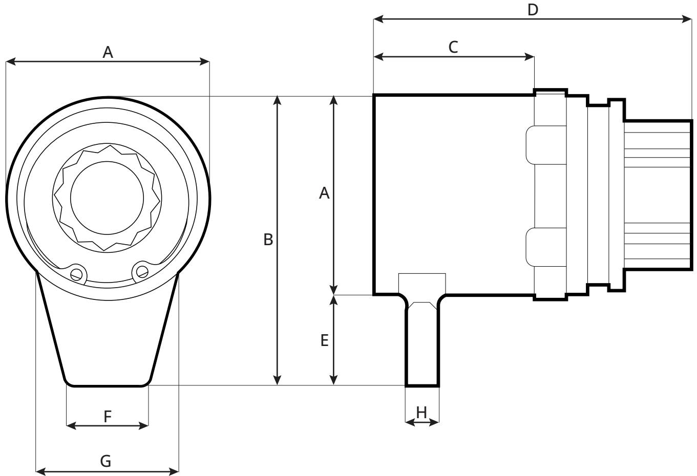
Bar Socket Dimensions for TN-39EZ Turn-of-Nut Wrench
