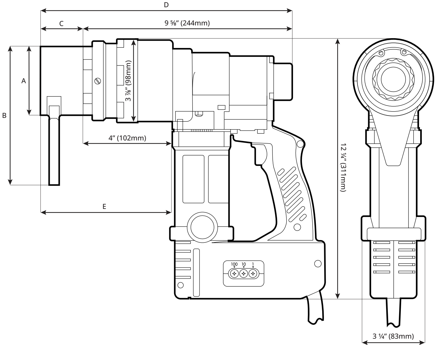
TN-33EZ Turn-of-Nut Wrench Dimensions w/ Bar Socket
