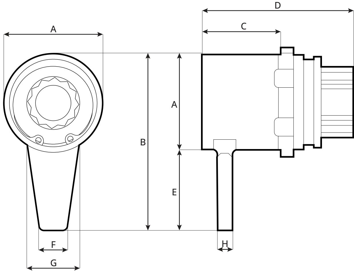
Bar Socket Dimensions for TN-33EZ Turn-of-Nut Wrench
