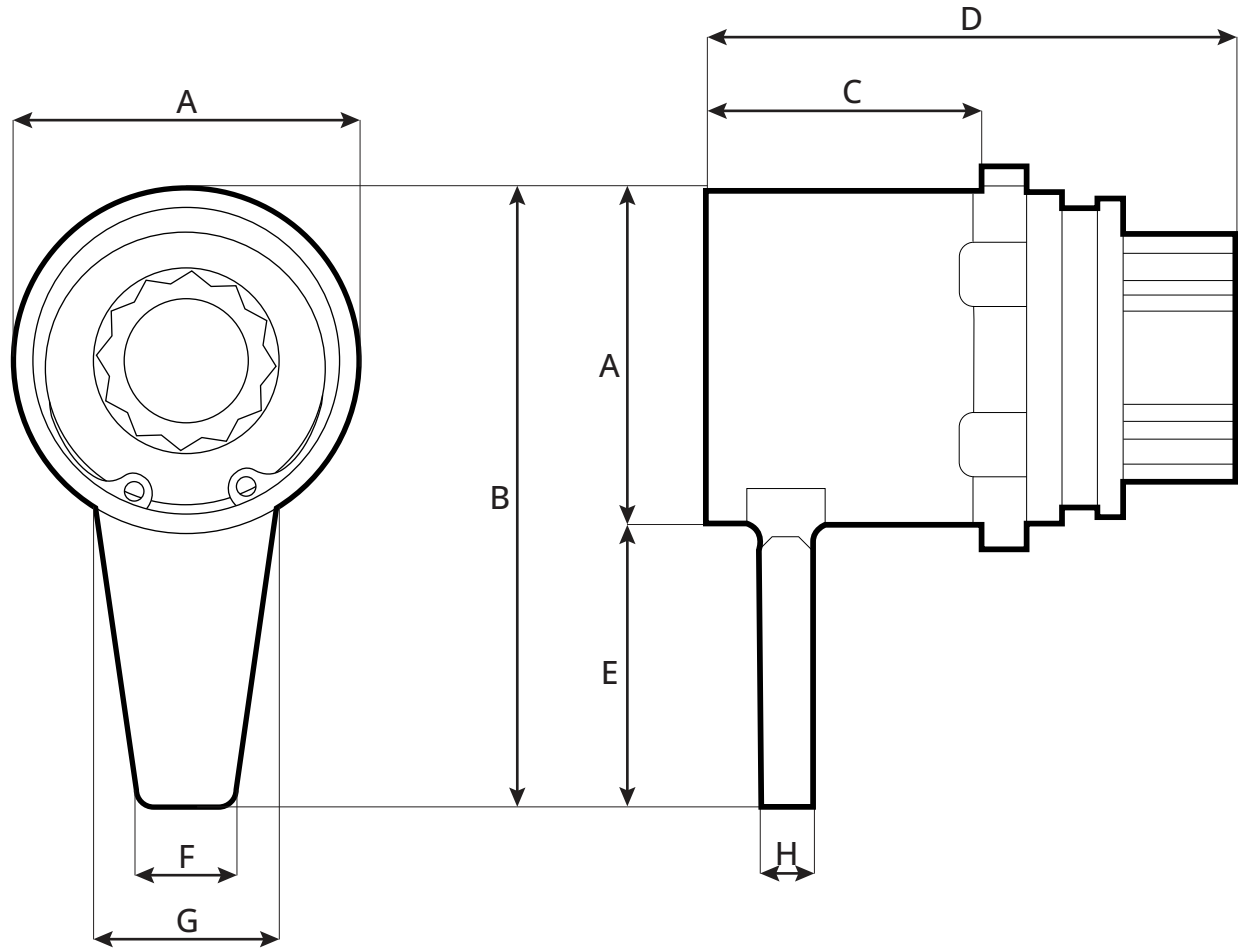
Bar Socket Dimensions for TN-30EZ Turn-of-Nut Wrench
