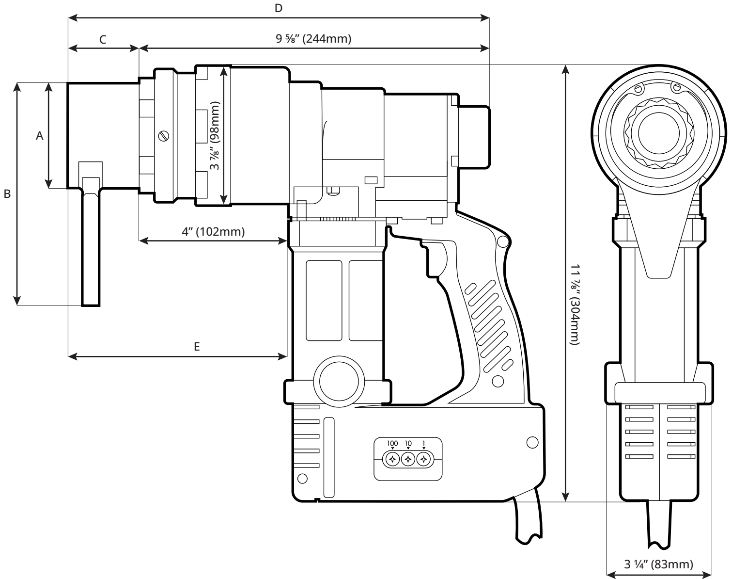
TN-30EZ Turn-of-Nut Wrench Dimensions w/ Bar Socket
