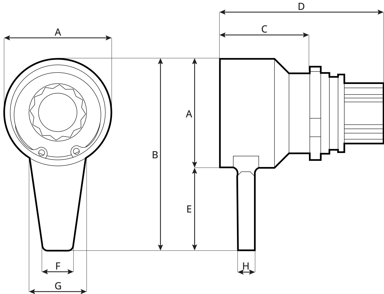
Bar Socket Dimensions for TN-24EZA Turn-of-Nut Wrench
