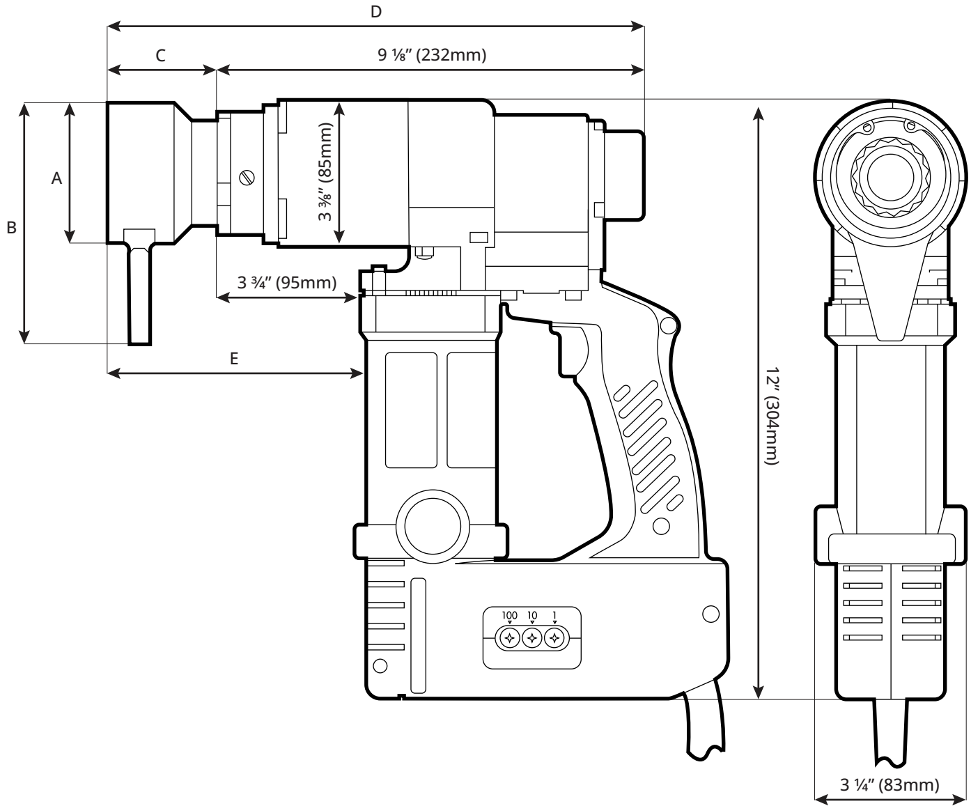
TN-24EZA Turn-of-Nut Wrench Dimensions w/ Bar Socket
