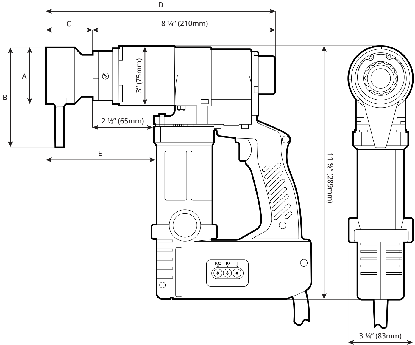
TN-22EZ Turn-of-Nut Wrench Dimensions w/ Bar Socket
