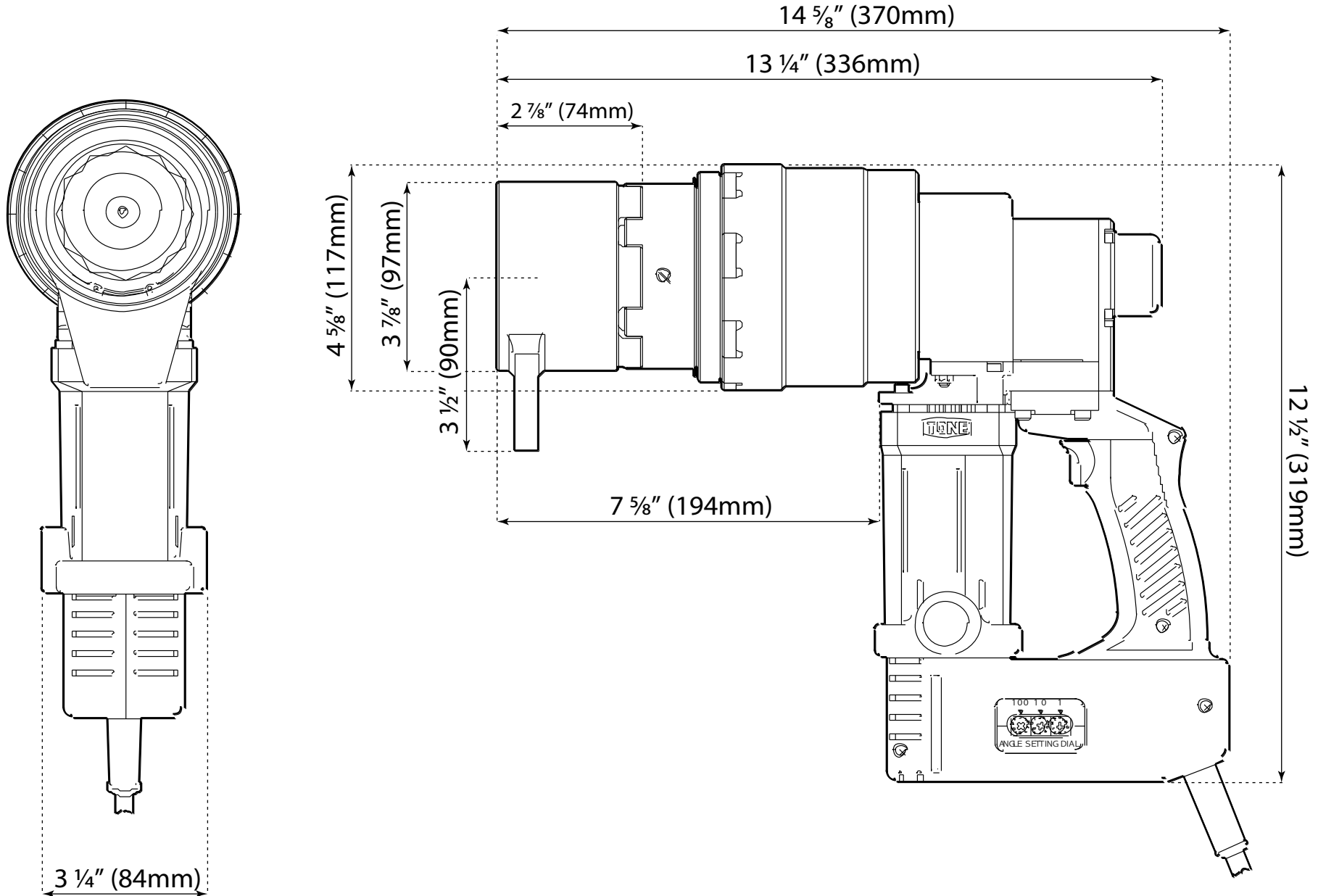
Dimensioned Drawing
