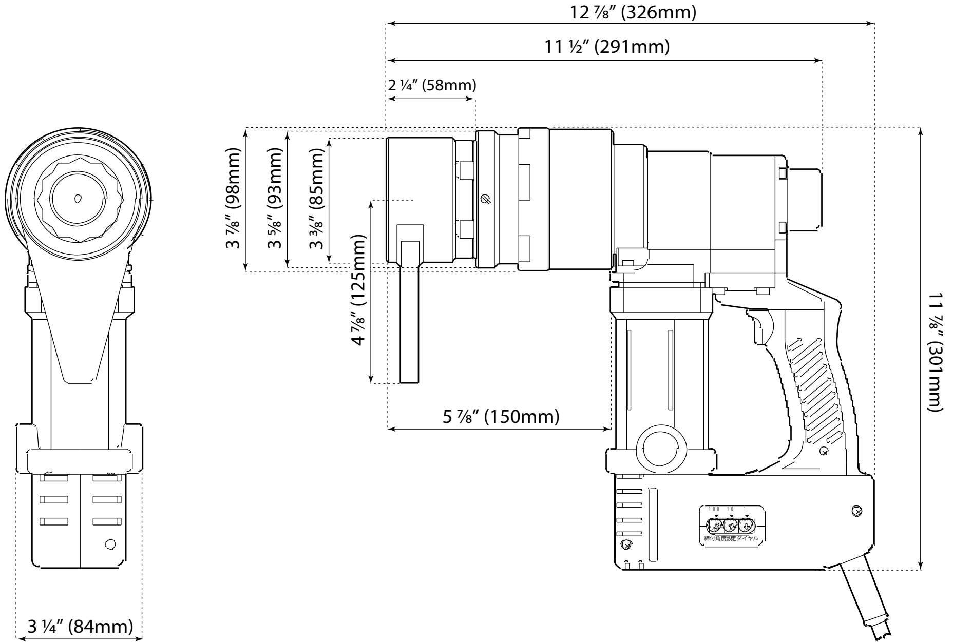
Dimensioned Drawing
