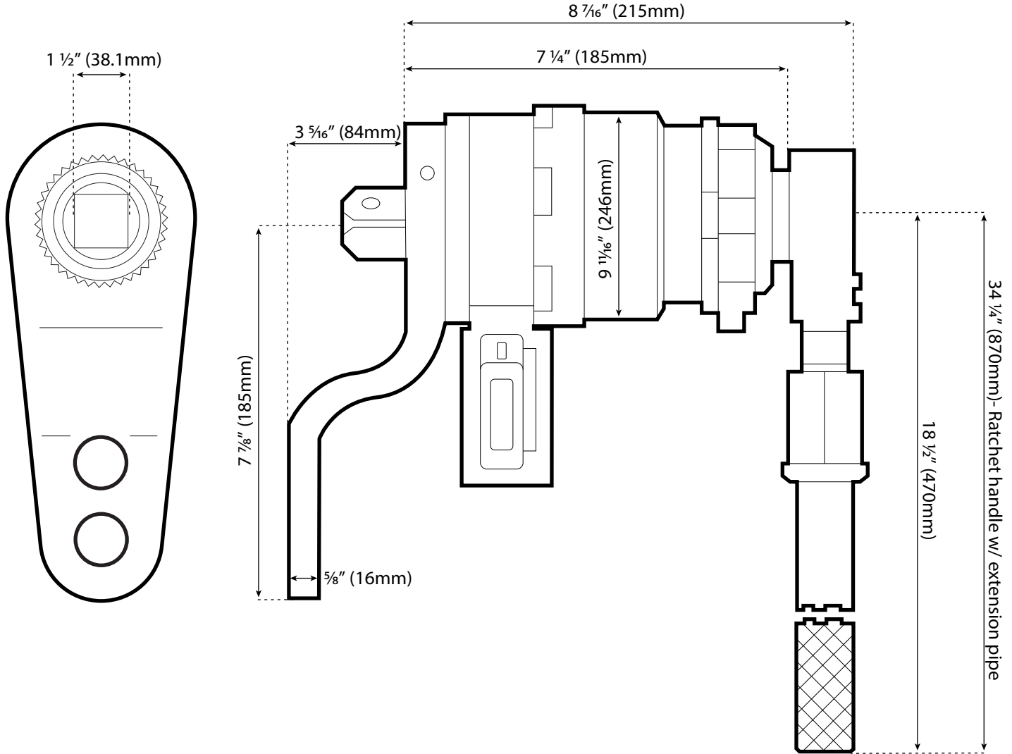
Dimensioned Drawing
