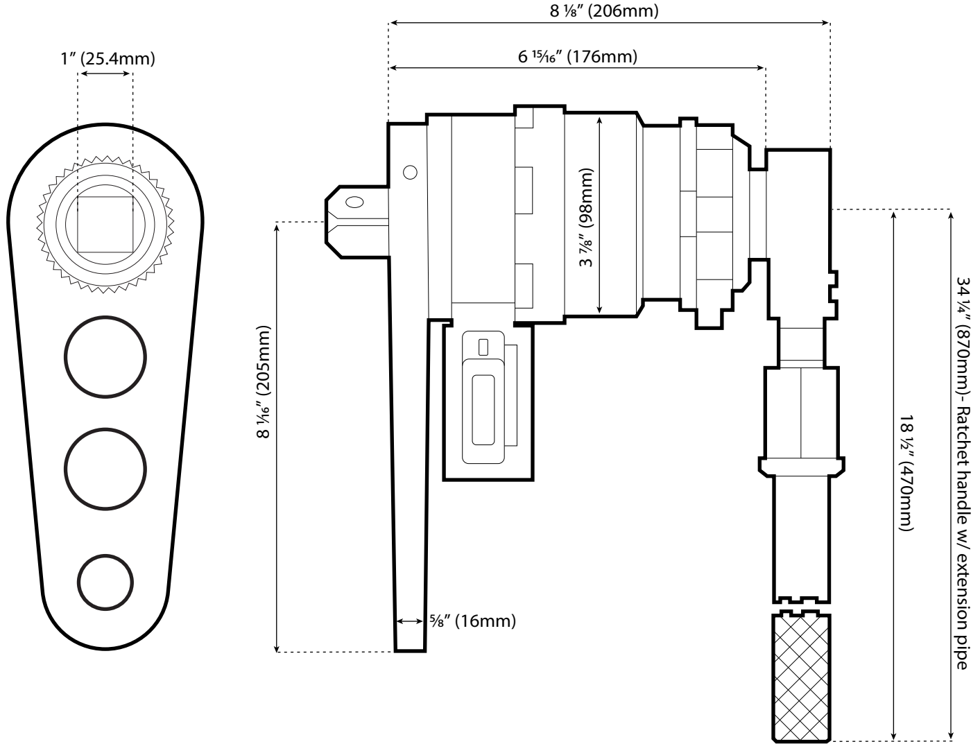
Dimensioned Drawing
