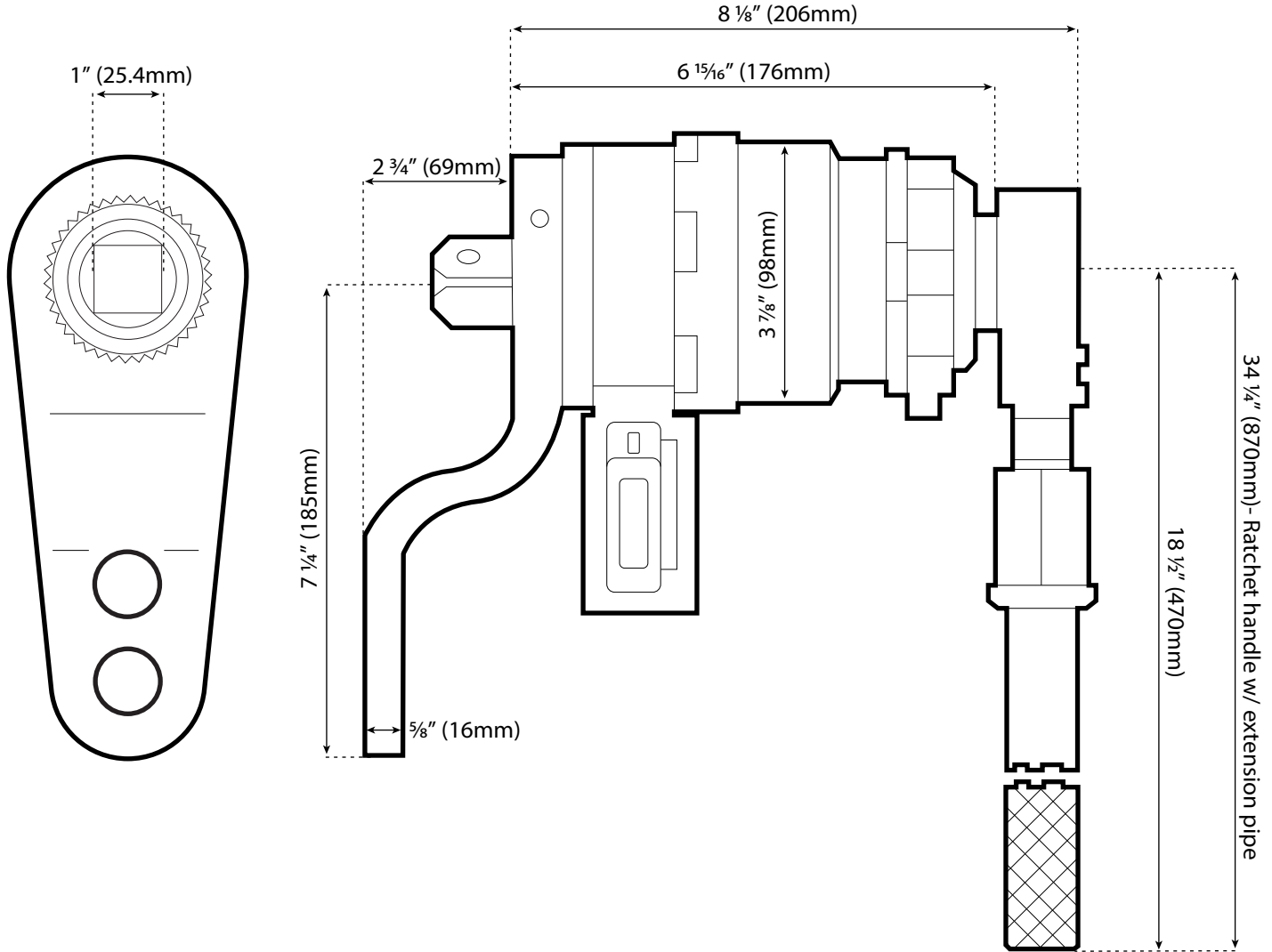
Dimensioned Drawing
