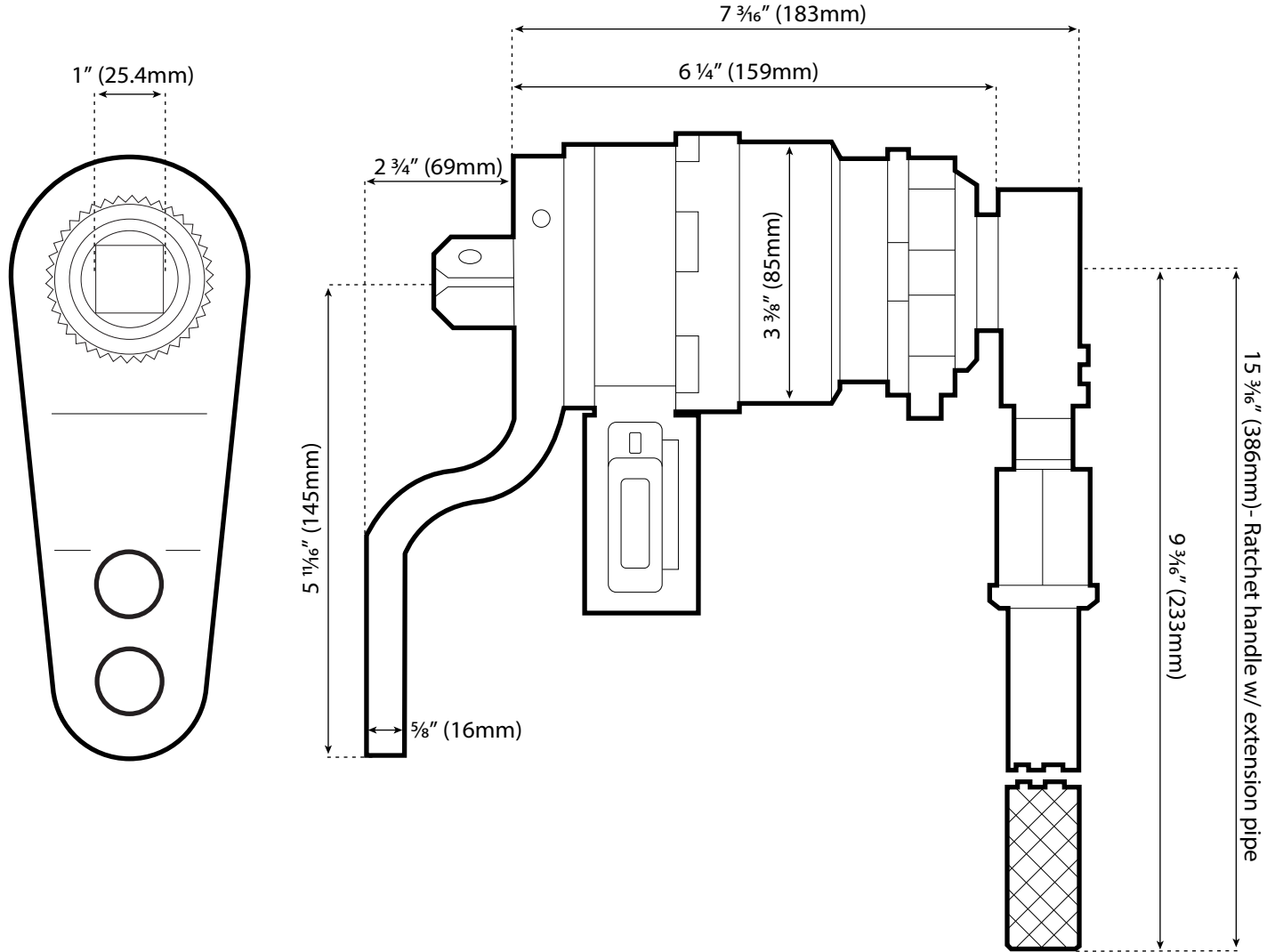
Dimensioned Drawing
