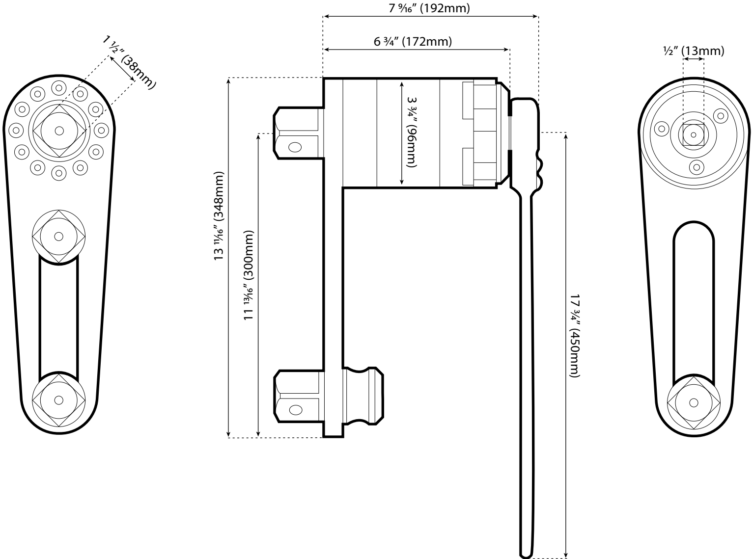
Dimensioned Drawing
