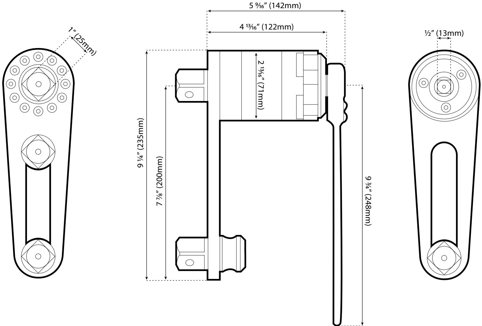
Dimensioned Drawing
